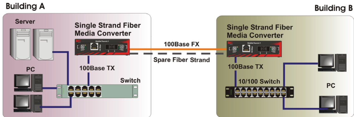
Figure 7: Single-strand fiber media converters using WDM technology can effectively double fiber capacity by combining wavelengths onto one strand of fiber. The spare fiber strand can immediately double the data traffic or be saved for future use.
