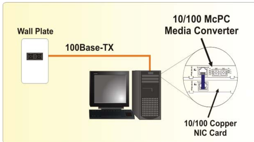
Figure 5: Media converters make FTTD a reality. Standalone or PC card media converters can be used at the desktop with standard 10/100 NICs to achieve further cost savings.
